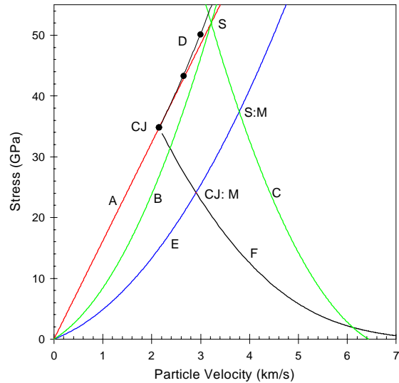
FIGURE 4. Hugoniots and isentropes relevant to calculating the reaction zone parameters. PBX 9501 is shown here. Explanations of the labels follow. (A) Detonation Rayleigh line. (B) Unreacted Hugoniot for the explosive. (C) Reflection of the unreacted Hugoniot for the explosive. (D) Explosive products Hugoniot. (E) PMMA window Hugoniot. (F) Explosives products isentrope calculated using the JWL EOS. (S) ZND spike point. (S:M) Spike point matched onto the PMMA Hugoniot. (CJ) Chapman-Jouguet or CJ state. (CJ:M) CJ state matched onto the PMMA Hugoniot. The matched spike and detonation points are those which would be observed.
